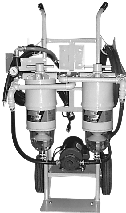
300-DHRAP5 Hydraulic Recycler Portable Unit
